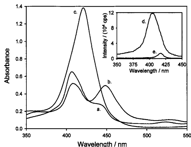
Figure 2. UV–visible absorption spectrum of a 15 \mu M solution of 1 in TFE after 43 days of incubation at 4 °C at (Soret band positions are noted in parentheses) (a) pH 8.01 (408 and 440 nm), (b) pH 6.37 (408 and 449 nm), and (c) pH 2.01 (420 nm). The inset shows the fluorescence excitation spectra of the solution from spectrum b monitored at (excitation band maxima are noted in parentheses) (d) 670 nm (404 nm) and (e) 600 nm (418 nm).
