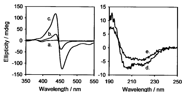
Figure 1. CD spectra of a 15 \mu M solution of 1 in TFE after storage at 4 °C and pH 7 for (a, d) 4 days, (b) 27 days, and (c, e) 101 days.
